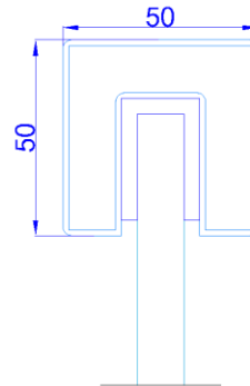
HRA50X50 SQUARE HANDRAIL
